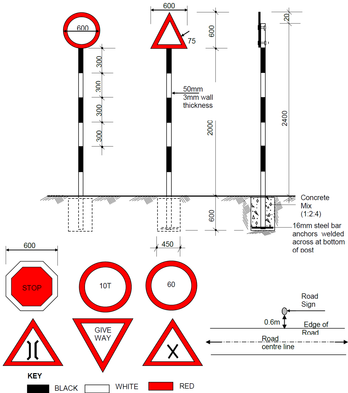
FIGURE C.16 - TRAFFIC SIGNS
