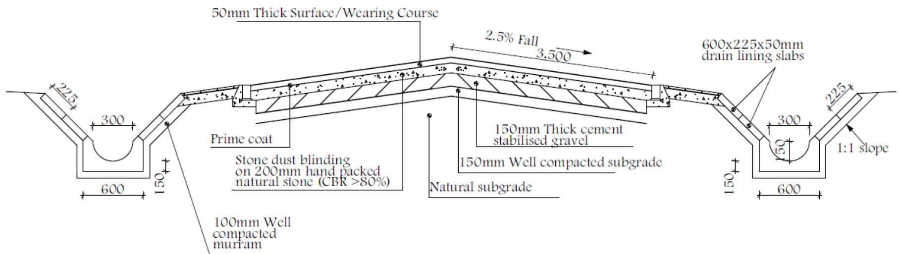
ROAD CROSS-SECTION
