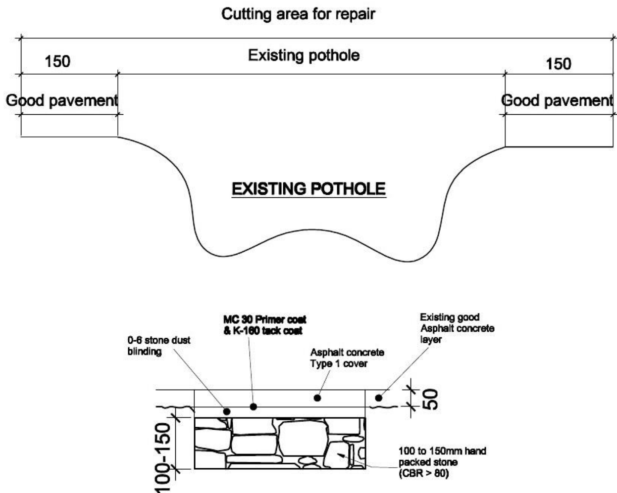
POTHOLE PATCHING FIG-P1
