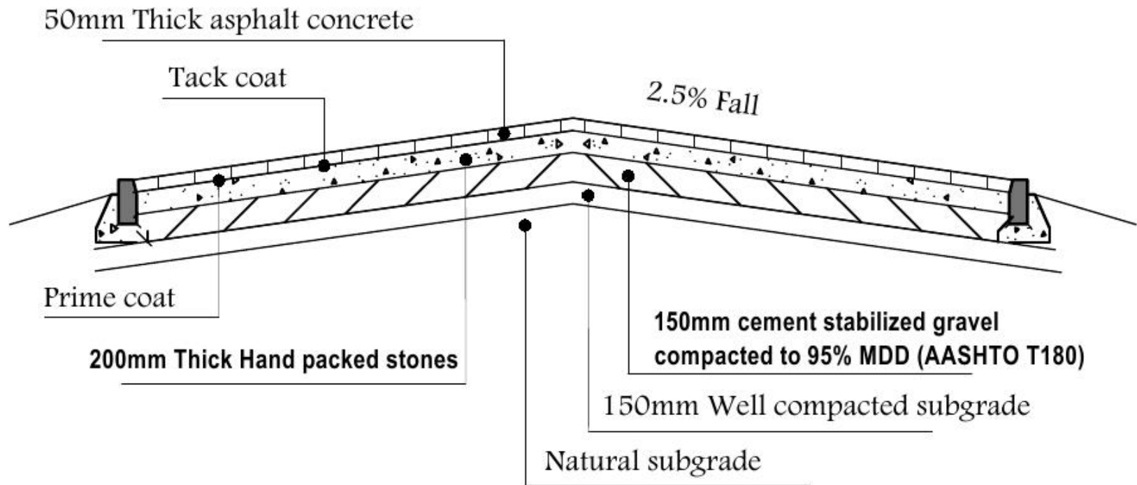
CROSS SECTION ~ ROAD FIG A
