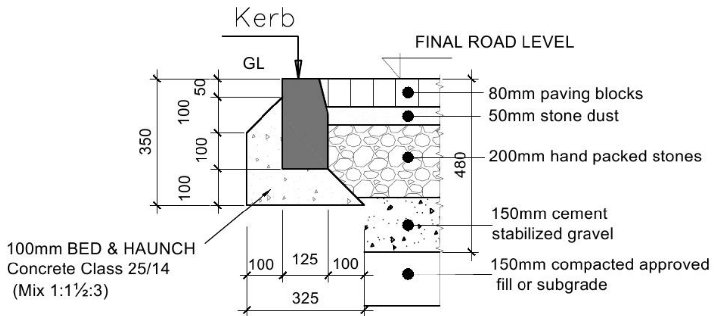
125X250mm KERB.-FIG K2
