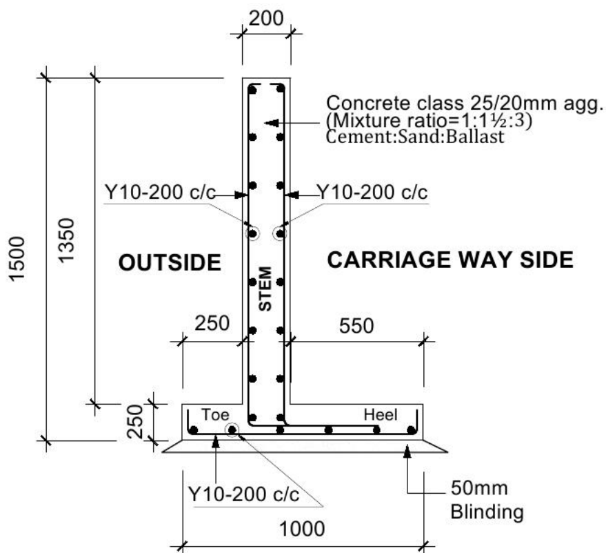
RETAINING WALL DETAIL FIGURE 3
