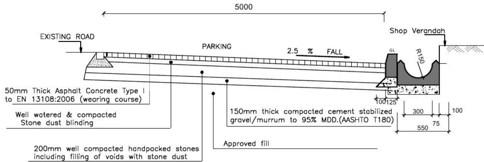
CROSS SECTION DETAIL. SCALE 1:50 VEHICLE PARKING -FIG-4
