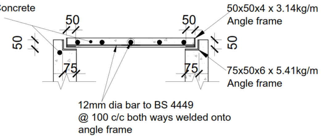
DRAIN COVER FIG.-DC- 1
