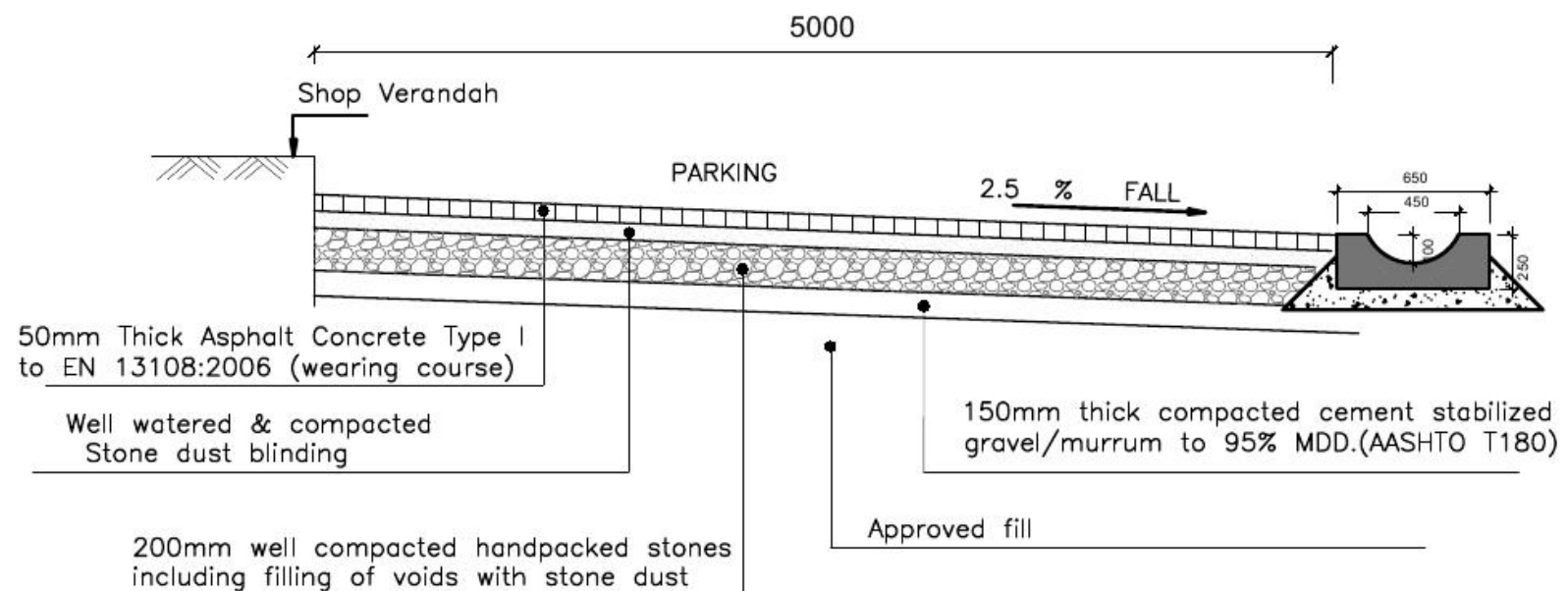
CROSS SECTION DETAIL. SCALE 1:50 VEHICLE PARKING -FIG-3
