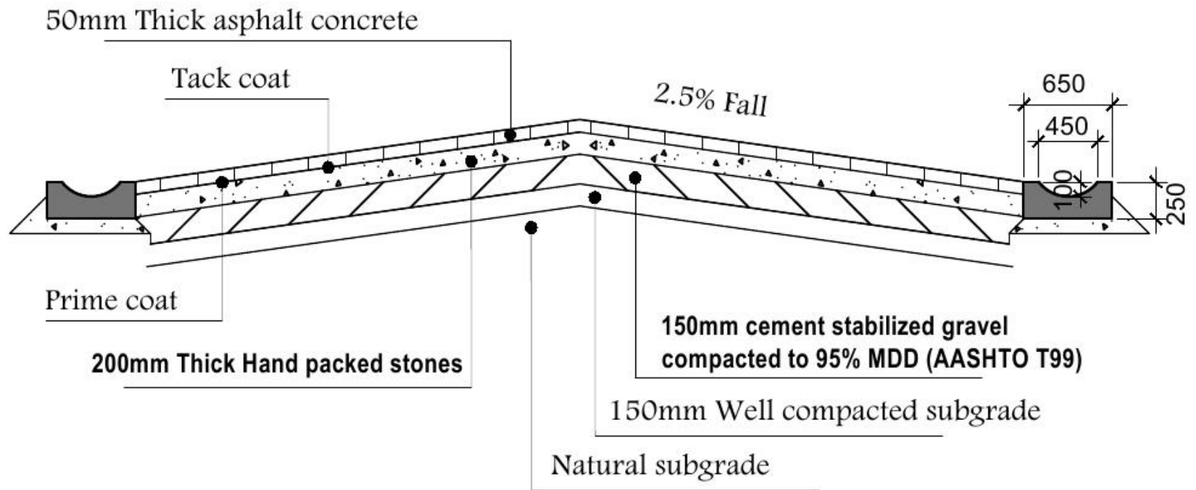
CROSS SECTION ~FIG C
