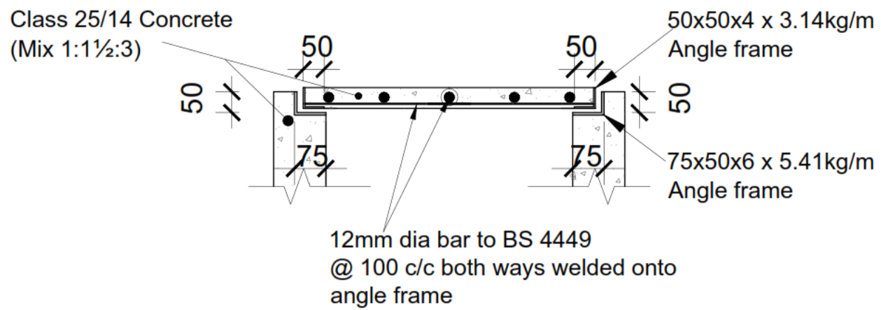
DRAIN COVER FIG.-DC- 1
