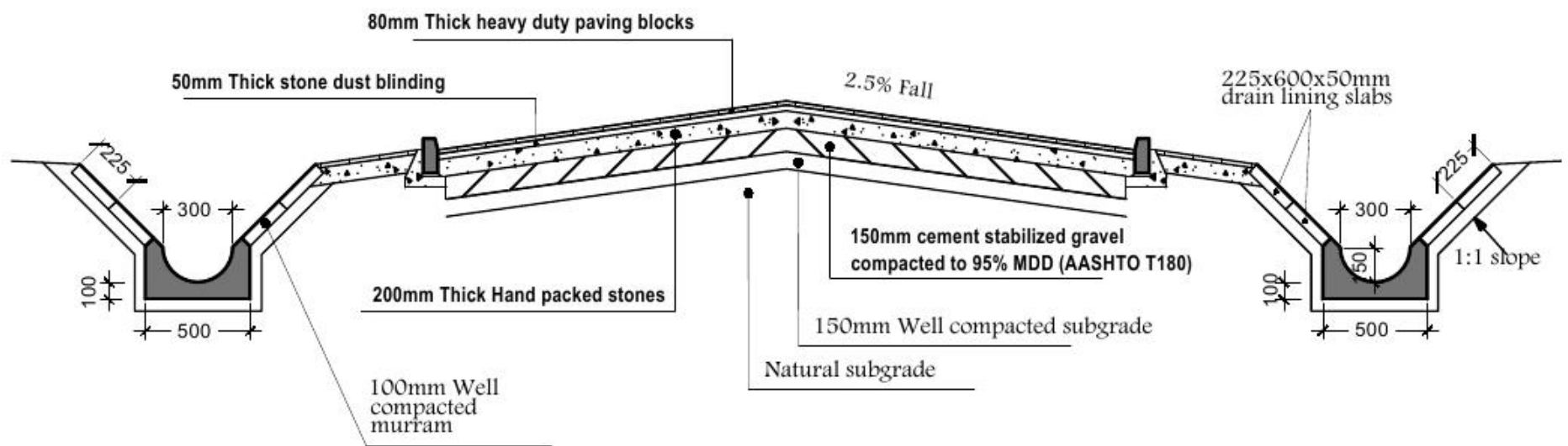
CROSS SECTION DETAIL-FIG B
