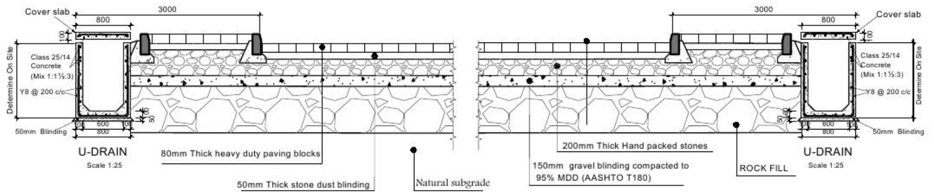
CROSS SECTION - MWEIGA BUS PARK: FIG M2
