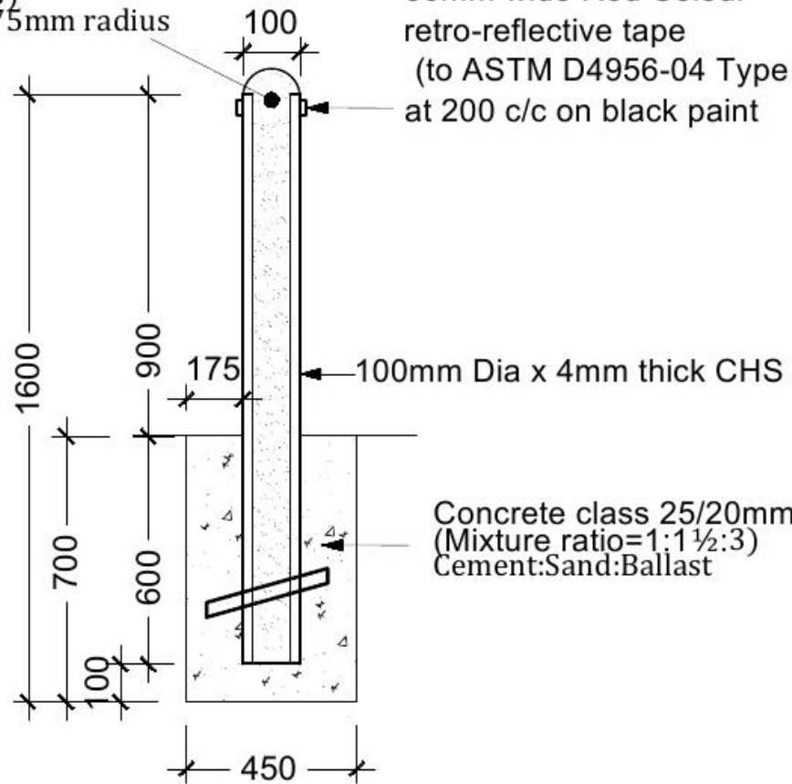
BOLLARD DETAIL FIGURE 4
