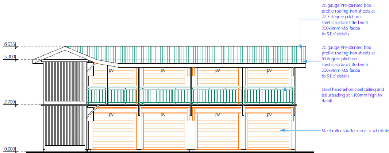
ELEVATION E-02 SCALE 1:100
