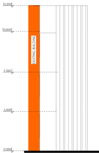
SIDE ELEVATION E-01 SCALE 1:100
