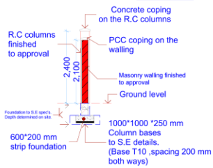
Columns and the wall details
